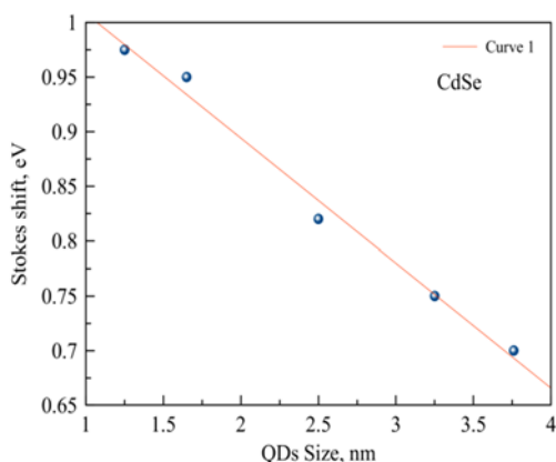
Figure 2: Dependence of the Stokes shift on the QDs size.
