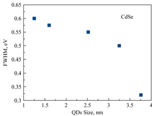
Figure 5: Dependence of the PL FWHM magnitudes for glasses doped with CdSe QDs with different sizes.
