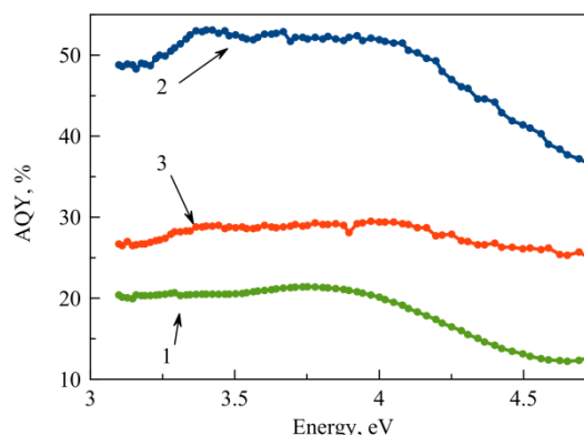
Figure 3: Dependence of the PL AQY for glasses doped with CdSe QDs with sizes 2.0 nm (1), 3.0 nm(2), 4.0 nm (3) on the excitation energy.
