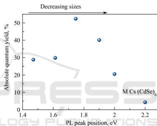
Figure 4: Dependence of the PL AQY on the CdSe QDs sizes.
