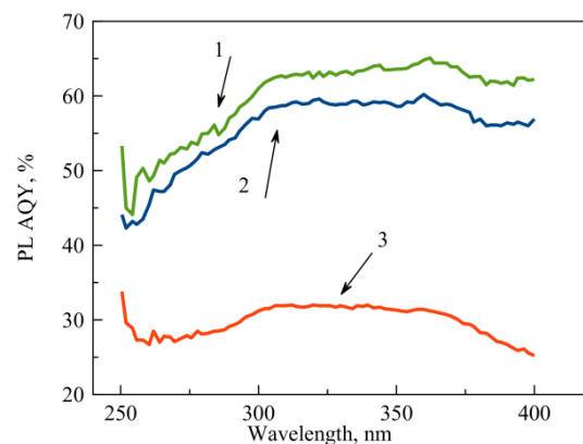
Figure 7: Dependence of PL AQY magnitudes for glasses doped with CdS QDs with sizes 2.3 nm (1), 3.5 nm (2) and 2.5 nm (3), respectively, on the excitation wavelength.
