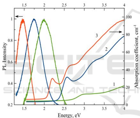
Figure 1: Absorption and luminescence spectra of the glass doped with CdSe QDs with a sizes 2.0 nm (1), 3.0 nm (2), 4.0 nm (3). The excitation energy is 3.06 eV.
