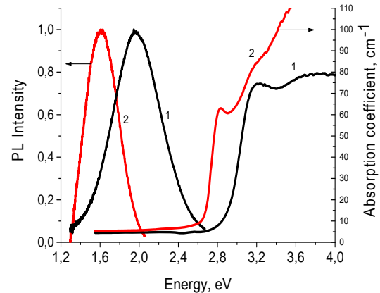
Figure 6: Absorption and luminescence spectra of the glasses doped with CdS QDs with sizes 2.3 nm (1), 3.5 nm (2). The excitation energy is 3.06 eV.
